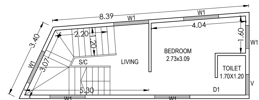
TYPICAL (FIRST & SECOND) FLOOR PLAN
